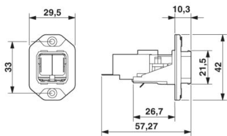
Push-Pull SCRJ panel mounting frame
