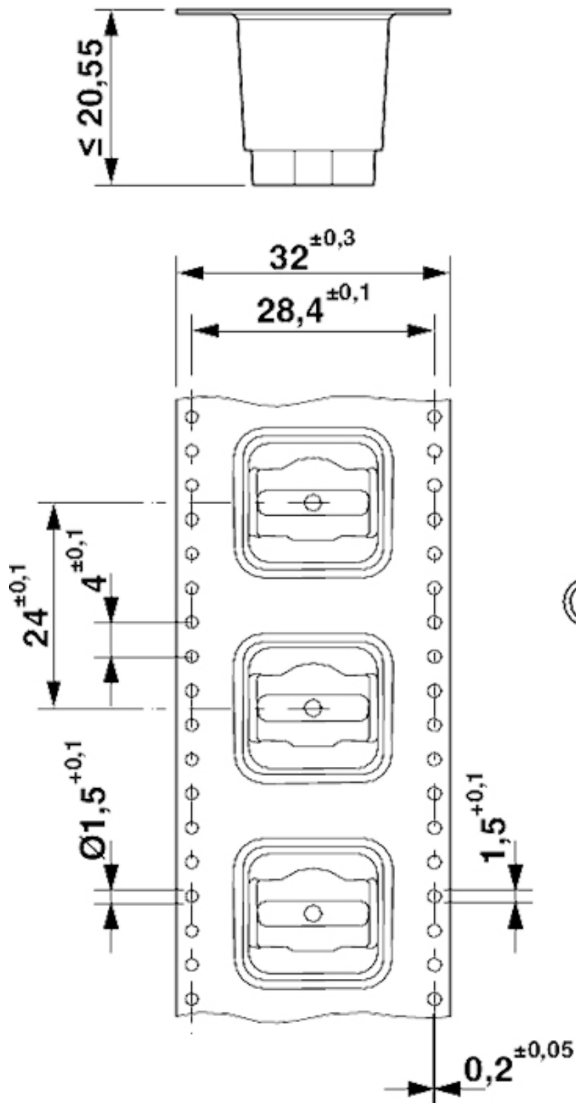
Dimensional drawing
