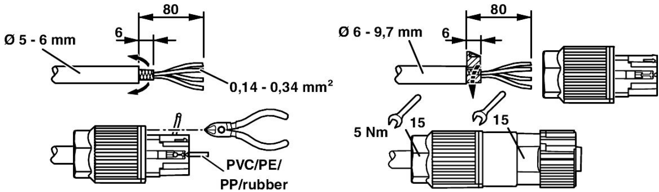
Functional drawing
