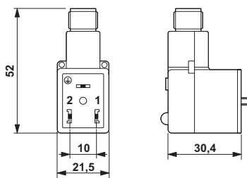
Valve connector, type B with horizontal M12 plug
