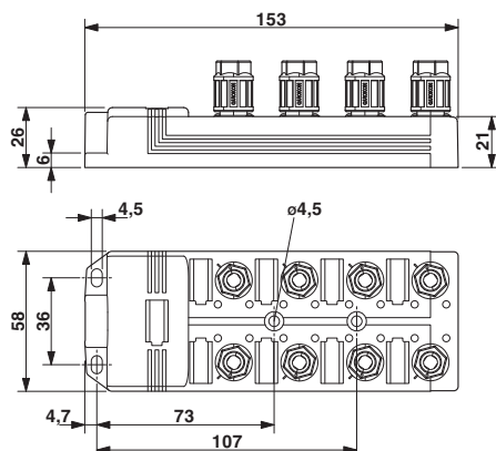
Dimensional drawing
