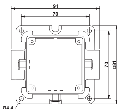
Dimensional drawing
