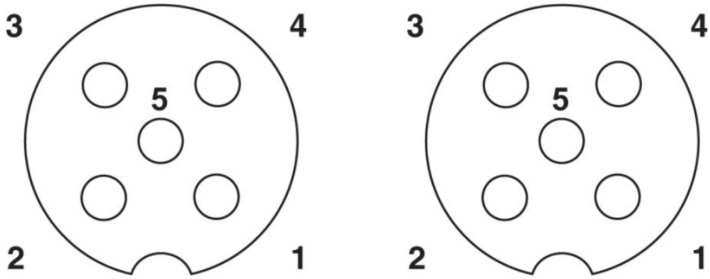
Pin assignment, female connector M 12 (female side)
