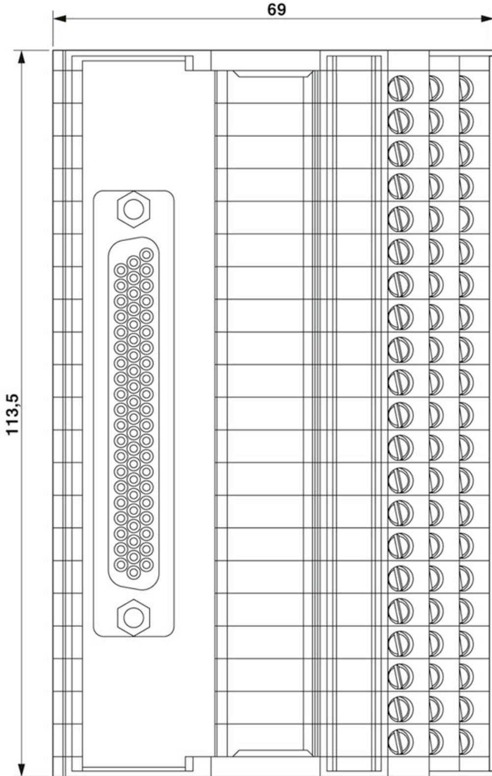
Dimensional drawing
