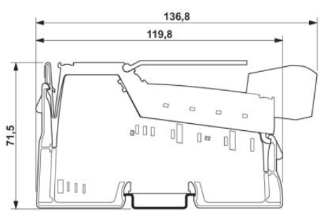
Dimensioned drawing
