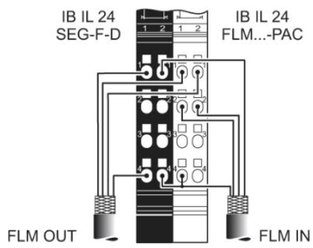
Connection diagram
