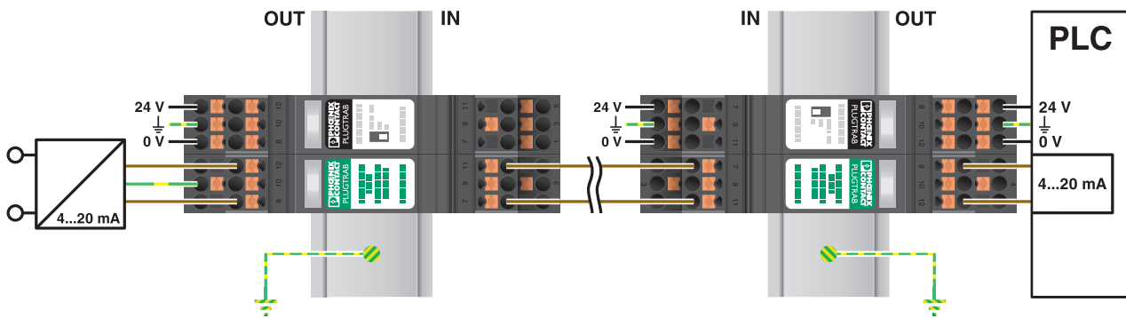
Application drawing
