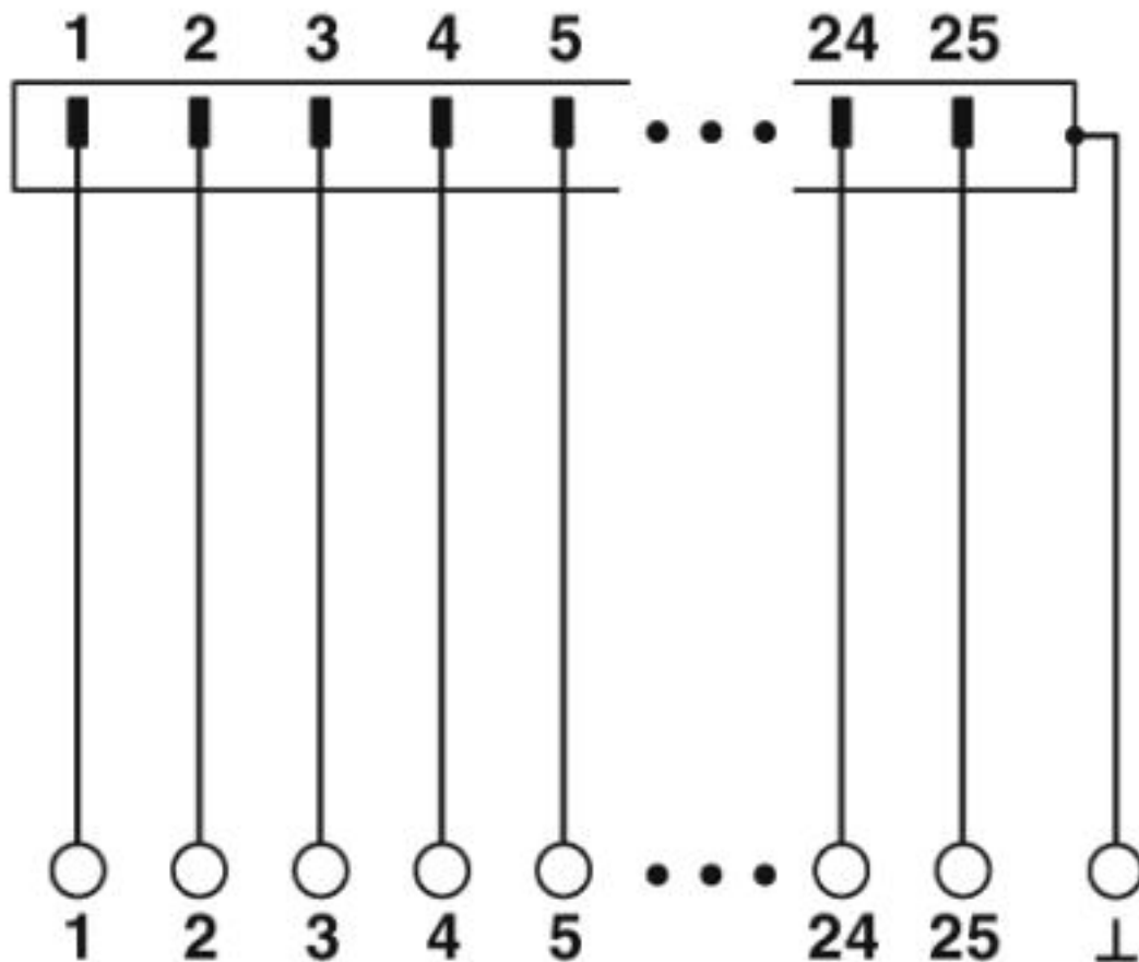
Circuit diagram
