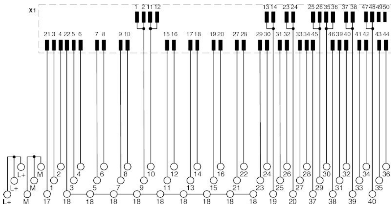
Circuit diagram
