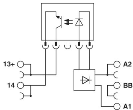
Circuit diagram
