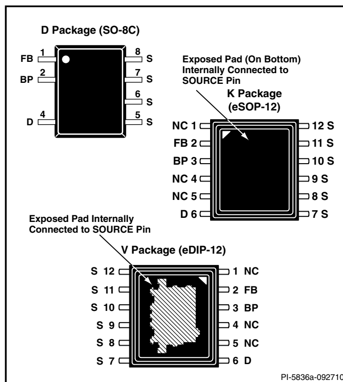
Figure 3. Pin Configuration (Top View).
