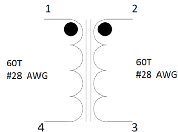
Figure 11 – Inductor Electrical Diagram.
