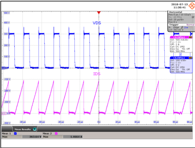
Figure 73 – Drain Voltage and Current Waveforms. 85 VAC, 20.0 V, 2.0 A Load (363 V MAX ). Upper: V DRAIN , 100 V / div., 20 μs / div. Lower: I DRAIN , 500 mA / div.
