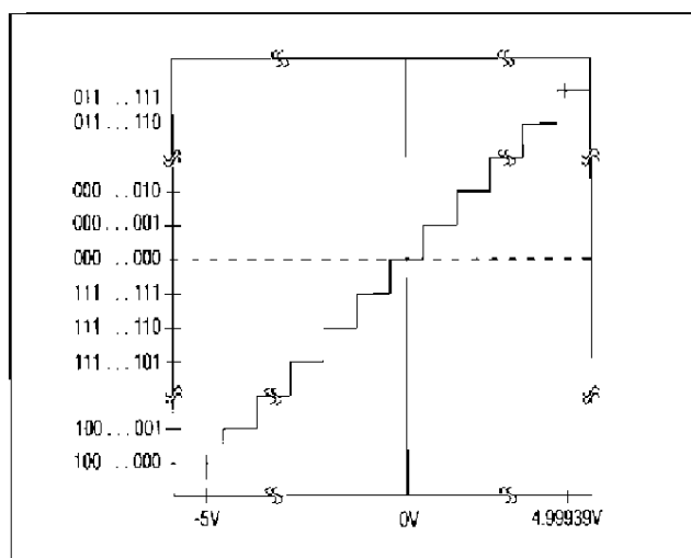
Figure 31. Bipolar Transfer Function
