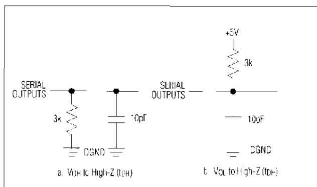
Figure 5 Load Circuits for Data-Hold Time
