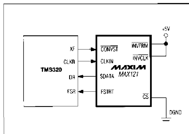
Figure 22. TMS320 Simple Serial-Interface Circuit
