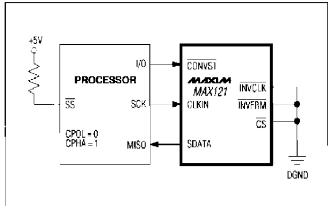
Figure 13. SPI Interface Circuit
