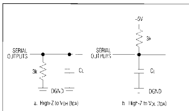
Figure 4 Load Circuits for Data-Access Time
