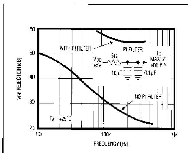
Figure 28. VDD Power-Supply Rejection vs. Frequency
