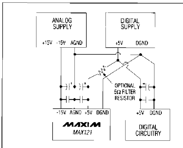
Figure 26. Power-Supply Grounding
