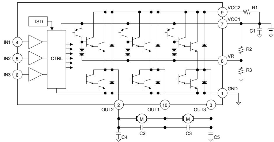
Fig.11 BA6238A
