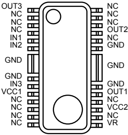
Fig.10 BA6247FP-Y (HSOP25)
