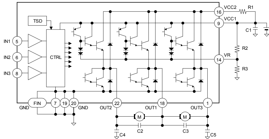
Fig.9 BA6247FP-Y
