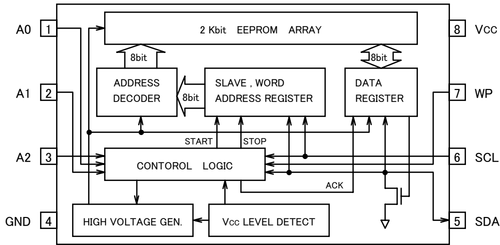
Fig.2 BLOCK DIAGRAM
