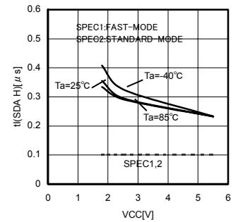
Fig.30 Noise Spike Width t_l(\text{SDA H})
