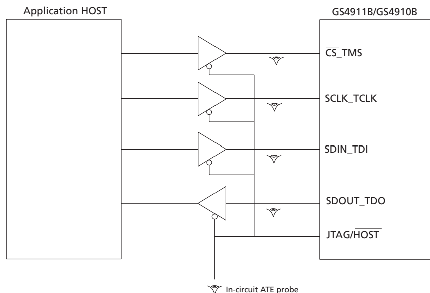
Figure 3-19: In-Circuit JTAG
