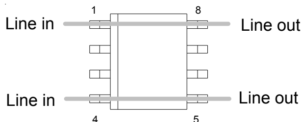
Connection for Differential Protection (Line-to-Line)
