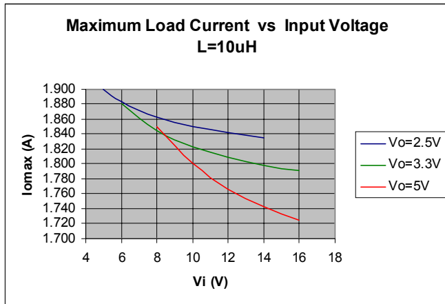
Figure 2. Theoretical maximum load current curves
