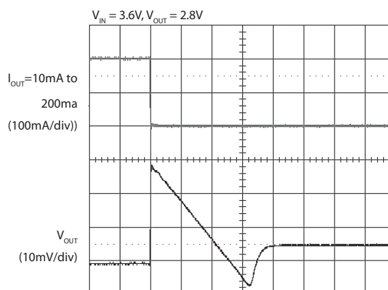
Load Transient Response Falling Edge (Both LDOs)
