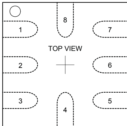
MLPQ-UT-8; 1.5x1.5, 8 LEAD \theta_{JA} = 157^{\circ}\text{C/W}
