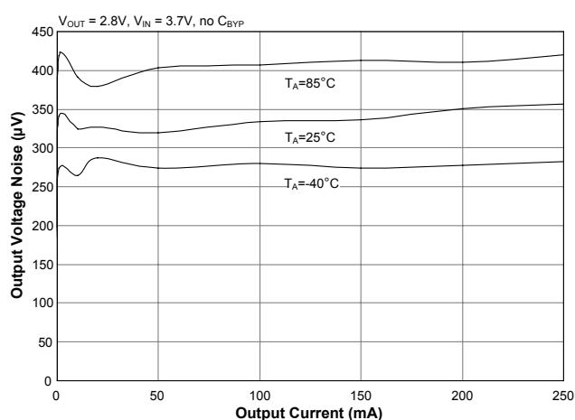
Output Noise vs. Load Current (Both LDOs)
