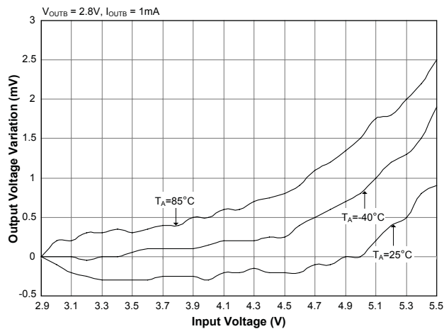
Line Regulation — LDOB
