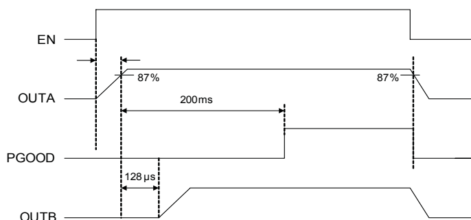
Figure 1 — Timing Diagram
