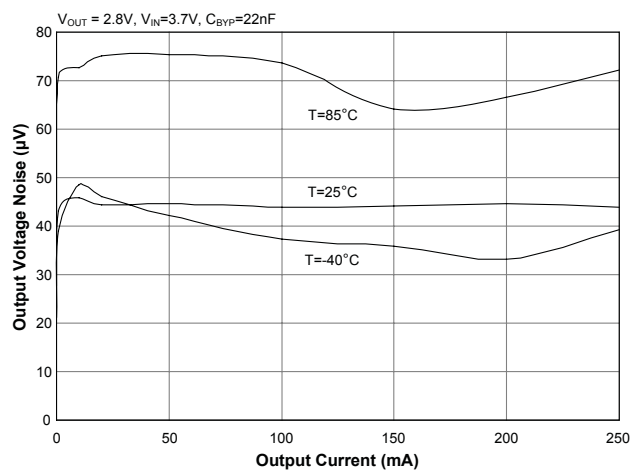
Output Noise vs. Load Current (Both LDOs)
