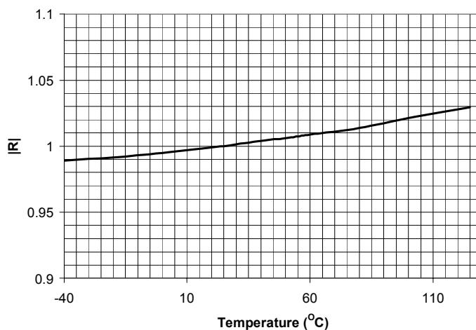
Normalized Resistance vs. Temperature
