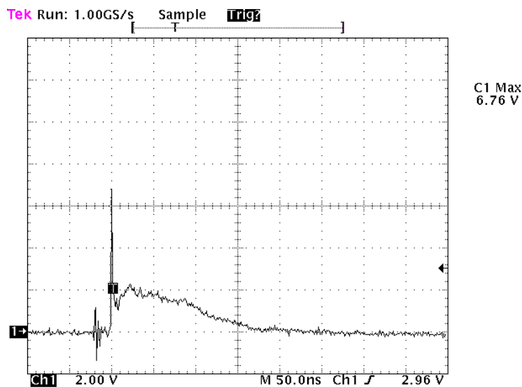
ESD Clamping (8kV Contact per IEC 61000-4-2)
