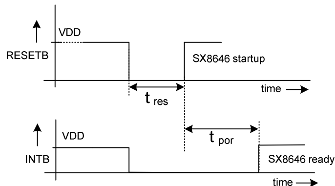
Figure 17 Hardware Reset
