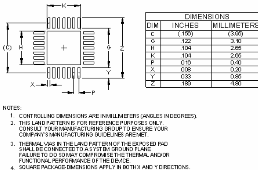
Figure 52 Land Pattern
