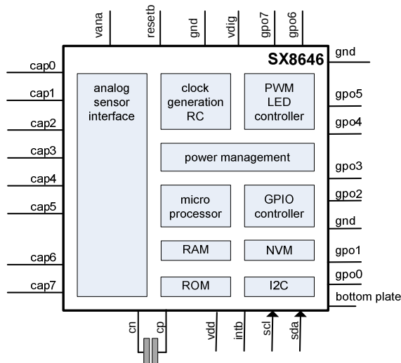
Figure 3 Simplified block diagram of the SX8646
