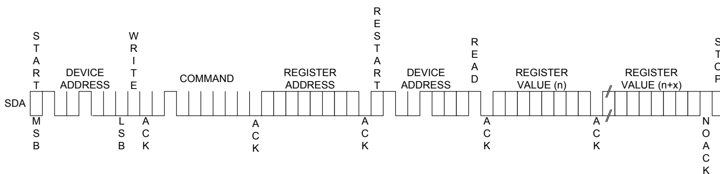
Figure 11. I2C frame: read burst register, command 0x30
