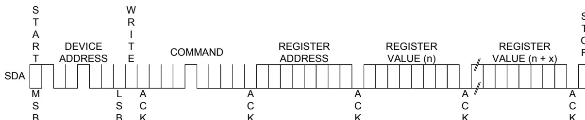
Figure 8. I2C frame: write burst register, command 0x10
