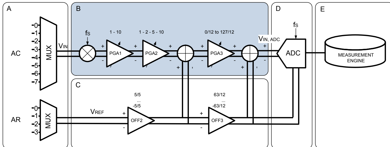
Figure 16. Programmable gain amplifiers (PGA) in the acquisition chain
