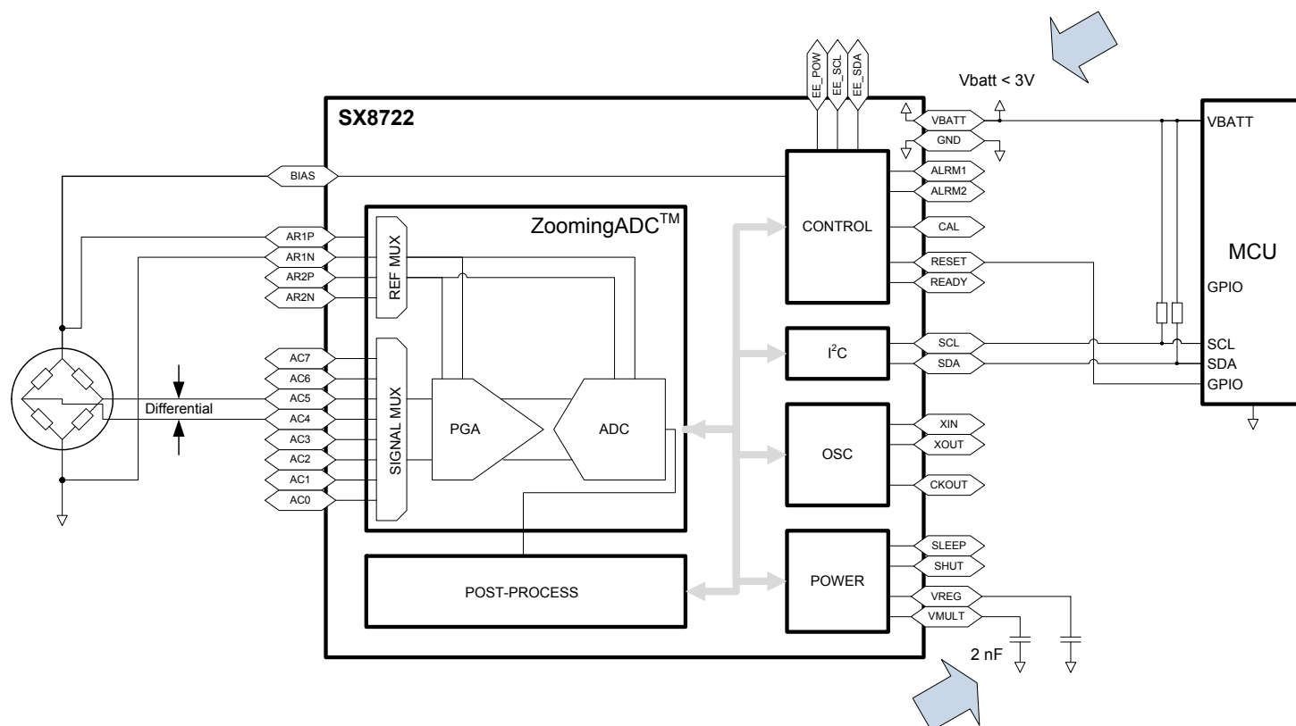
Figure 30. SX8722 working below 3V schematic
