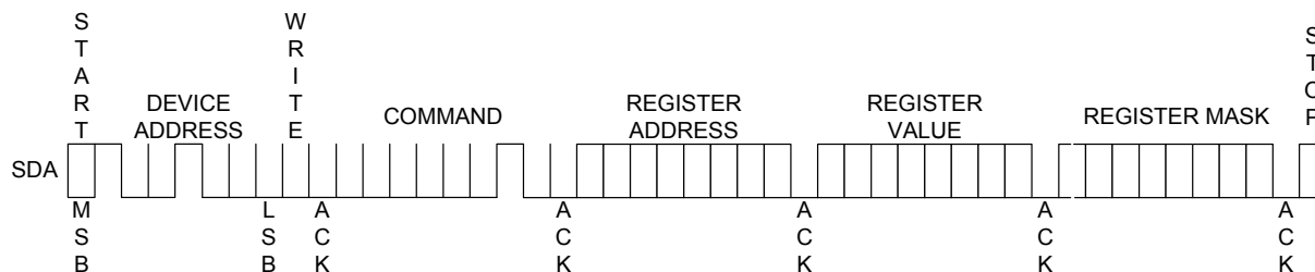
Figure 9. I2C frame: write mask register, command 0x20
