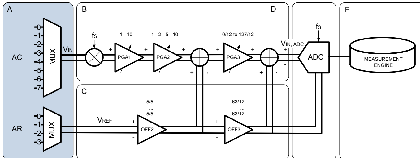
Figure 15. Input multiplexer overview
