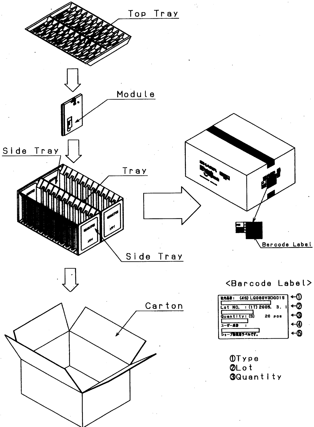
Fig.3 Packaging
