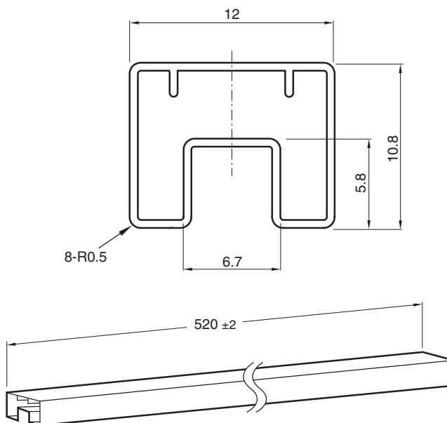
Fig. 3 Sleeve Shape and Dimensions
