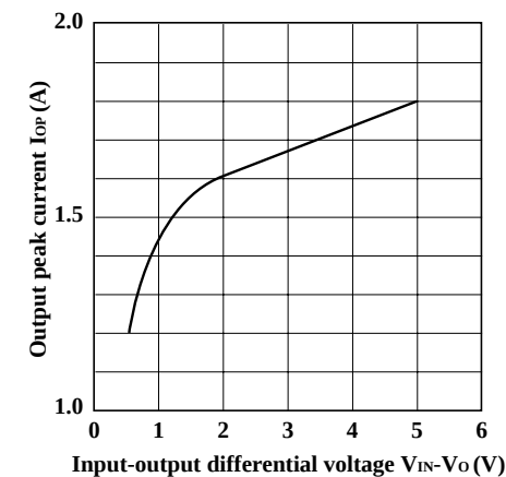
Fig.19 Output Peak Current vs. Input-output Differential Voltage
