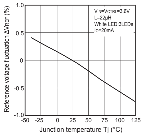
Fig.3 Reference Voltage Fluctuation vs. Junction Temperature
