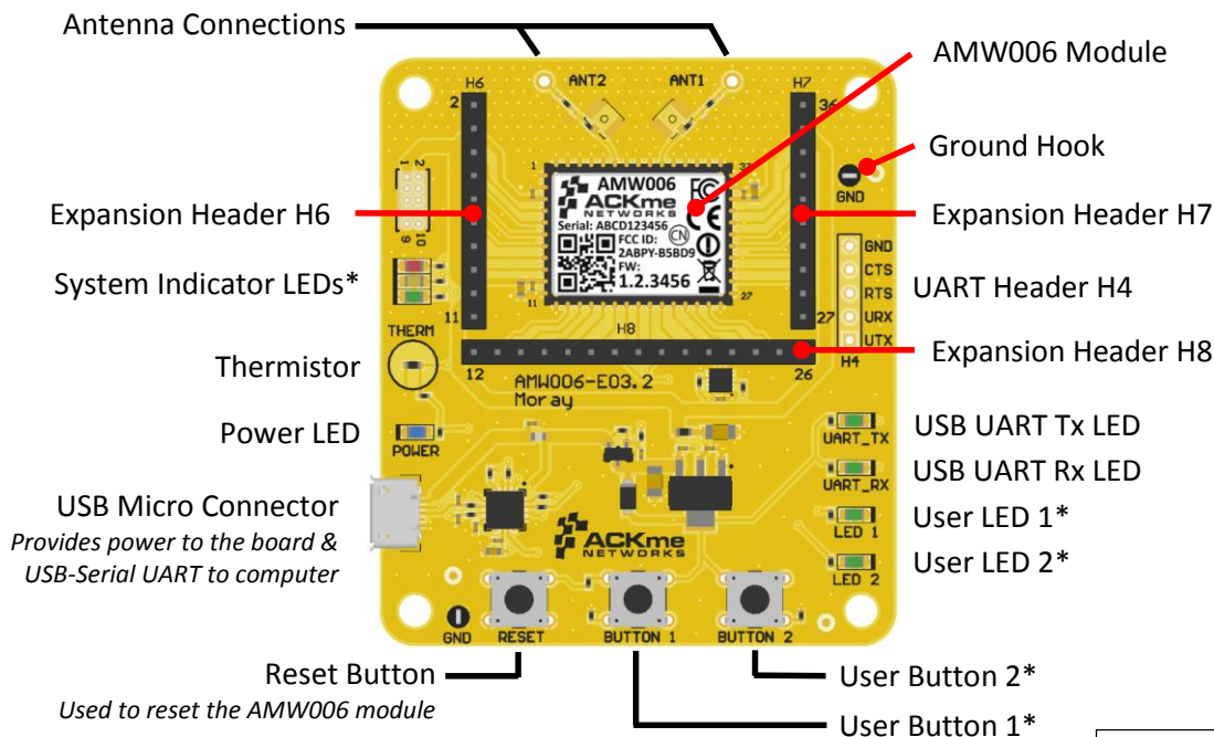
Figure 2. AMW006-E03 Features
