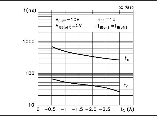
Figure 9. Resistive load switching off
