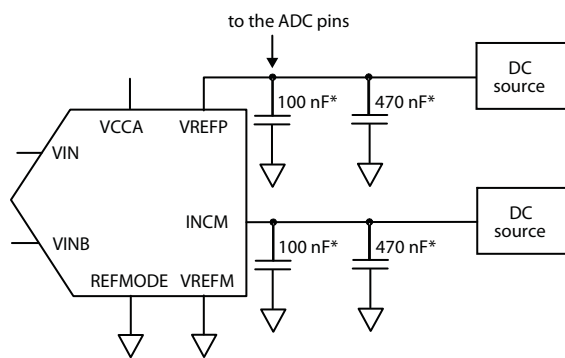
Figure 22. External voltage reference setting
