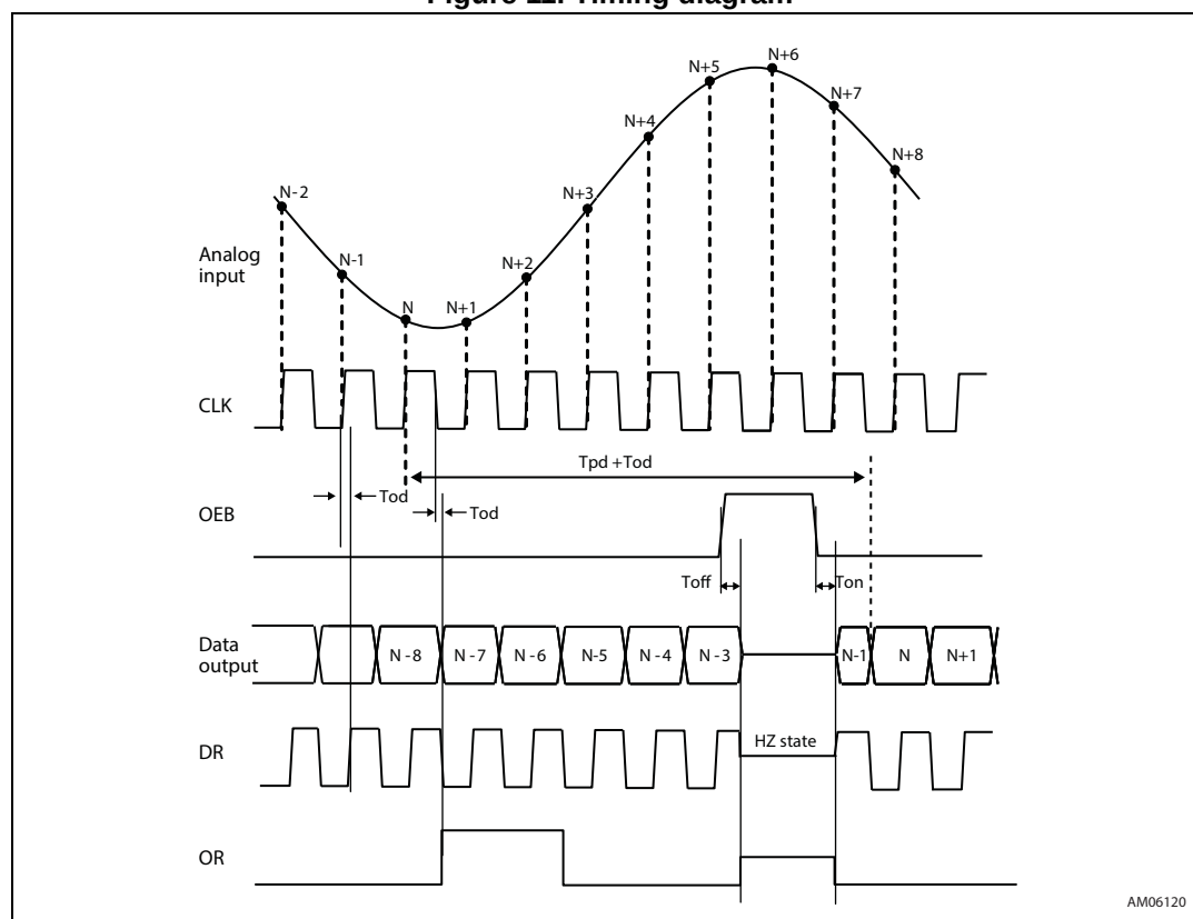
Figure 11. Timing diagram
