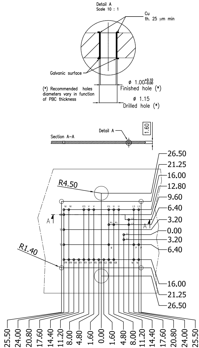
Figure 23. ACEPACK™ 2 CIB press fit pins recommended PCB holes layout (dimensions are in mm)
