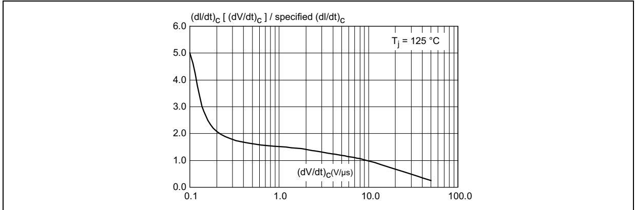
Figure 14. Relative variation of critical rate of decrease of main current versus reapplied (dV/dt)
