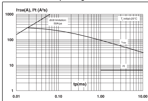
Figure 15. Non repetitive surge peak on-state current for a sinusoidal pulse with width t_p < 10 ms, and corresponding value of I^2t .
