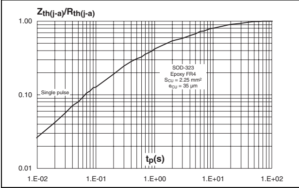
Figure 7. Relative variation of thermal impedance junction to ambient versus pulse duration (epoxy FR4 with recommended pad layout, e_{CU} = 35 \mu m ) (SOD-323)
