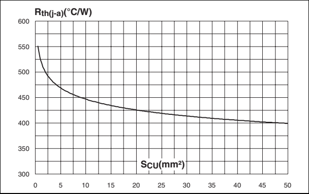
Figure 8. Thermal resistance junction to ambient versus copper surface under each lead (printed circuit board, epoxy FR4, e_{CU}=35 \mu m , SOD-323)
