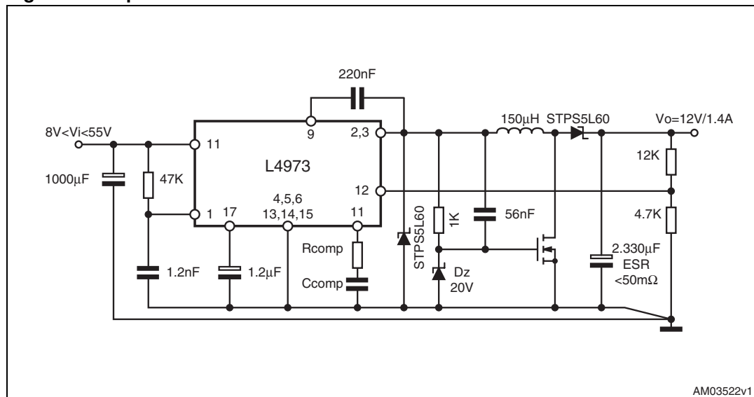
Figure 40. Up/down converter
