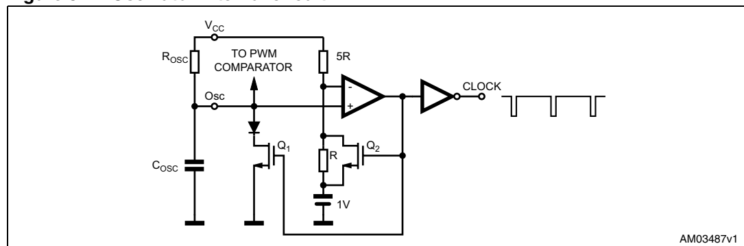
Figure 5. Oscillator internal circuit
