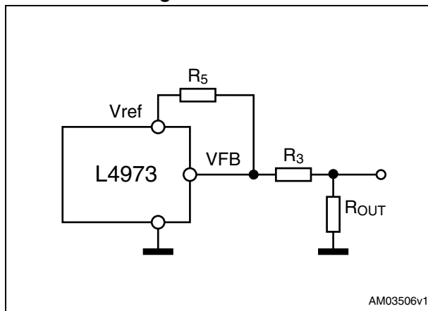
Figure 24. Example of output regulated voltage lower than 3.3 V
