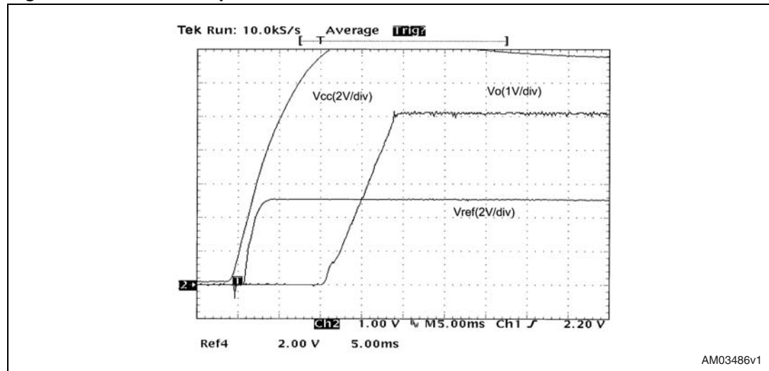
Figure 4. Turn-on sequence
