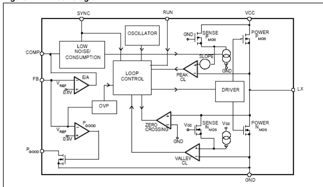
Figure 4. Block diagram
