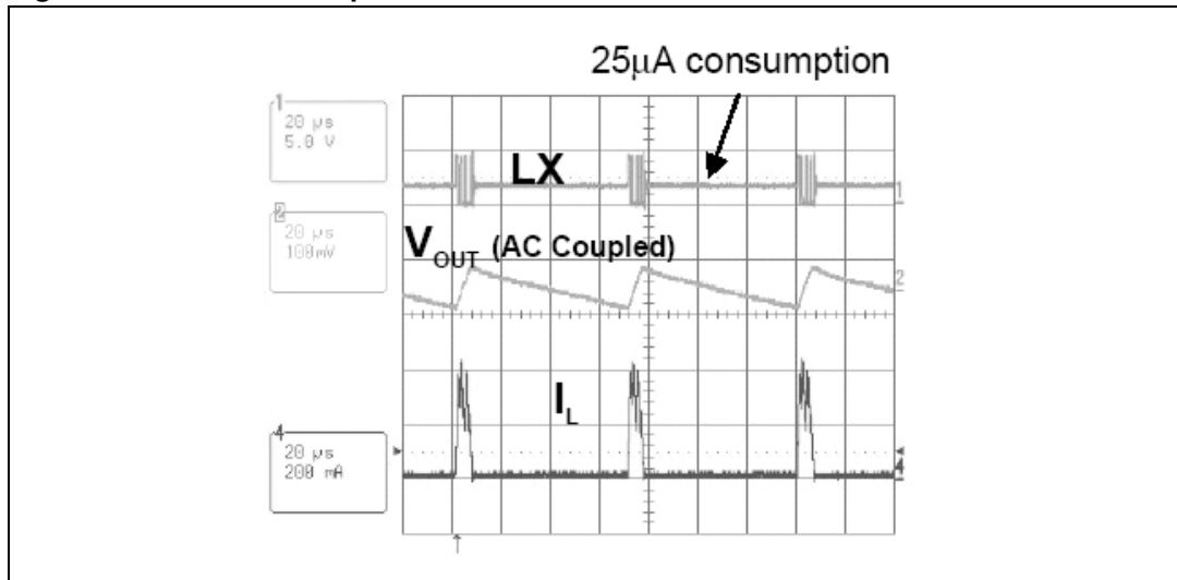
Figure 5. Low consumption mode
