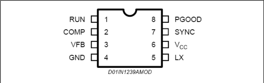
Figure 2. Pins connection
