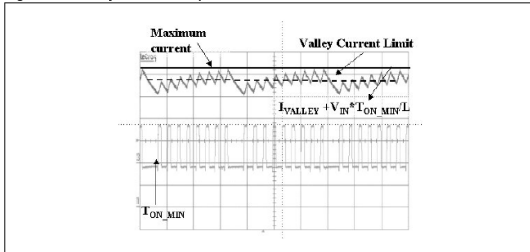
Figure 11. Valley current limit protection
