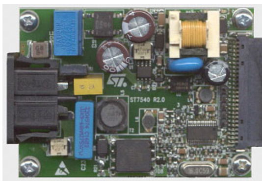
Figure 12. ST7540 reference design board (Rev 2.0)
