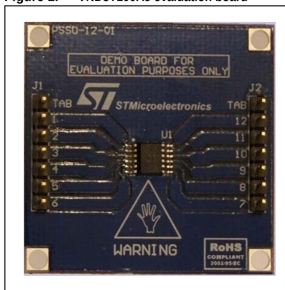
Figure 1. VND5T100AJ evaluation board
