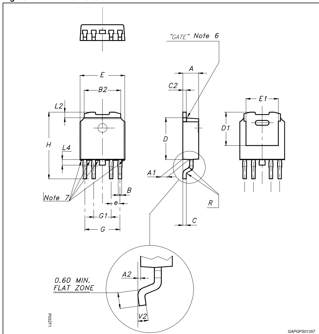
Figure 24. PPAK dimension
