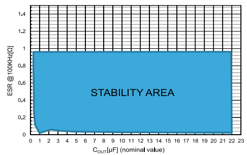
Figure 17: Stability area vs (COUT, ESR)
