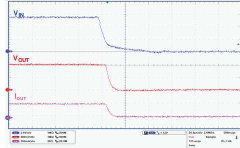
Figure 21: Turn-off time ( V_{OUT} = 1\text{ V} )
