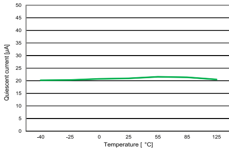
Figure 8: Quiescent current vs. temperature ( I_{OUT} = 0 \text{ mA} )
