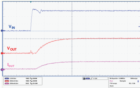
Figure 20: Turn-on time ( V_{OUT} = 1\text{ V} )
