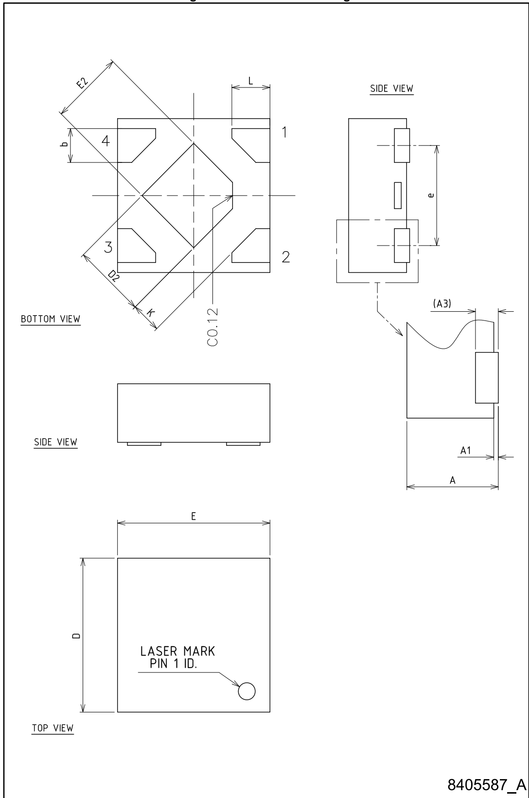
Figure 28: DFN 1x1-4L drawing
