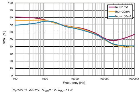
Figure 14: Supply voltage rejection vs. frequency
