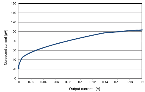
Figure 11: Quiescent current vs. load current
