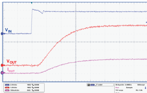
Figure 22: Turn-on time ( V_{OUT} = 5\text{ V} )
