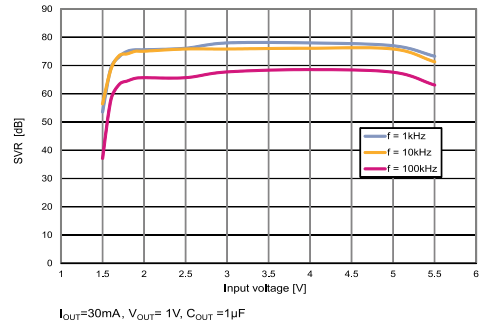
Figure 15: Supply voltage rejection vs. input voltage
