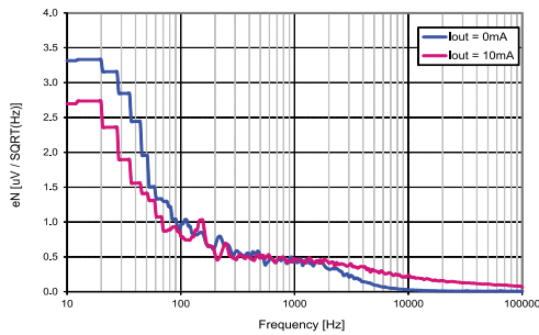
Figure 16: Output noise spectral density
