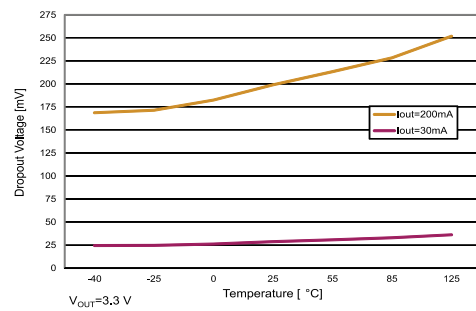
Figure 13: Dropout voltage vs. temperature
