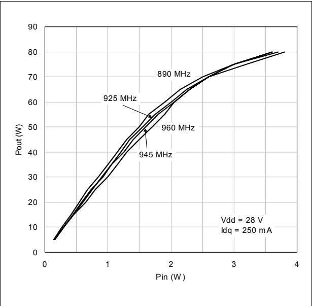
Figure 5. Output power vs input power
