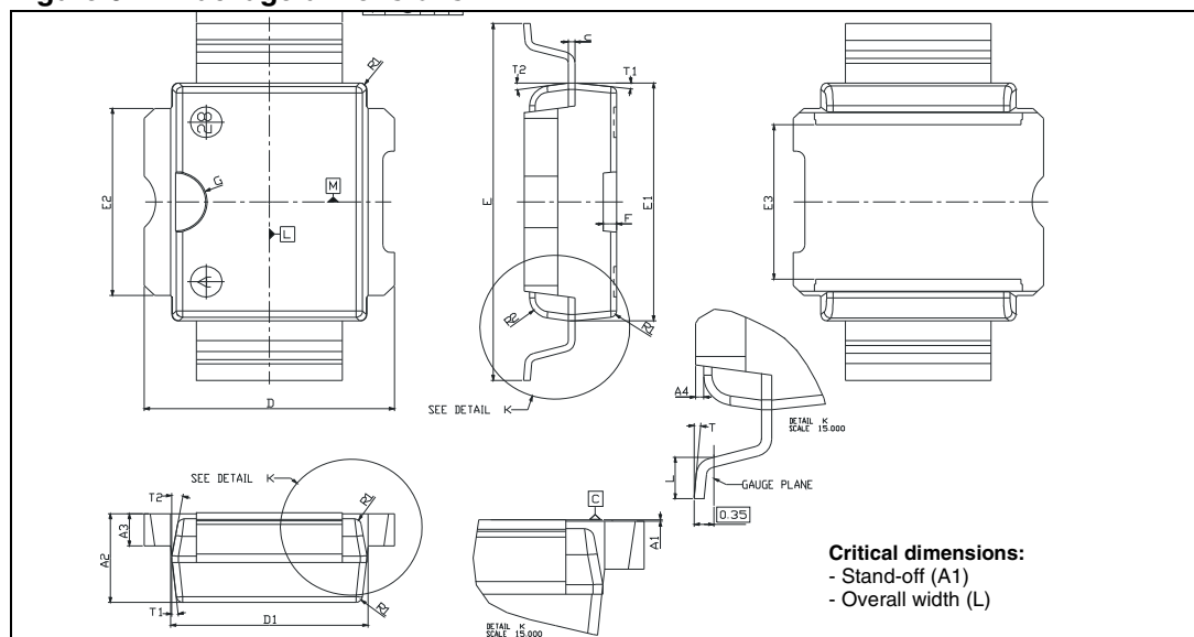
Figure 6. Package dimensions
