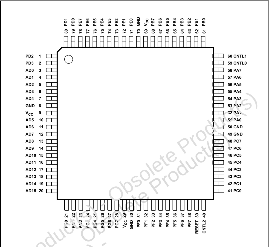
Figure 3. LQFP connections
