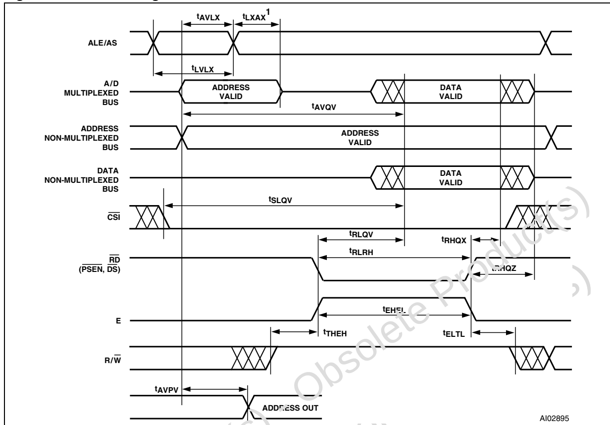
Figure 35. READ timing
