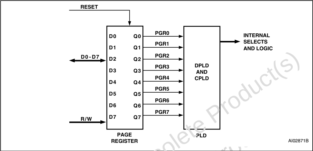
Figure 11. Page register
