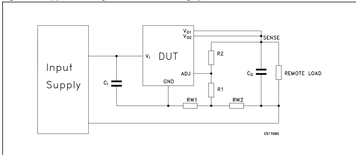
Figure 3. Application diagram for remote sensing operation
