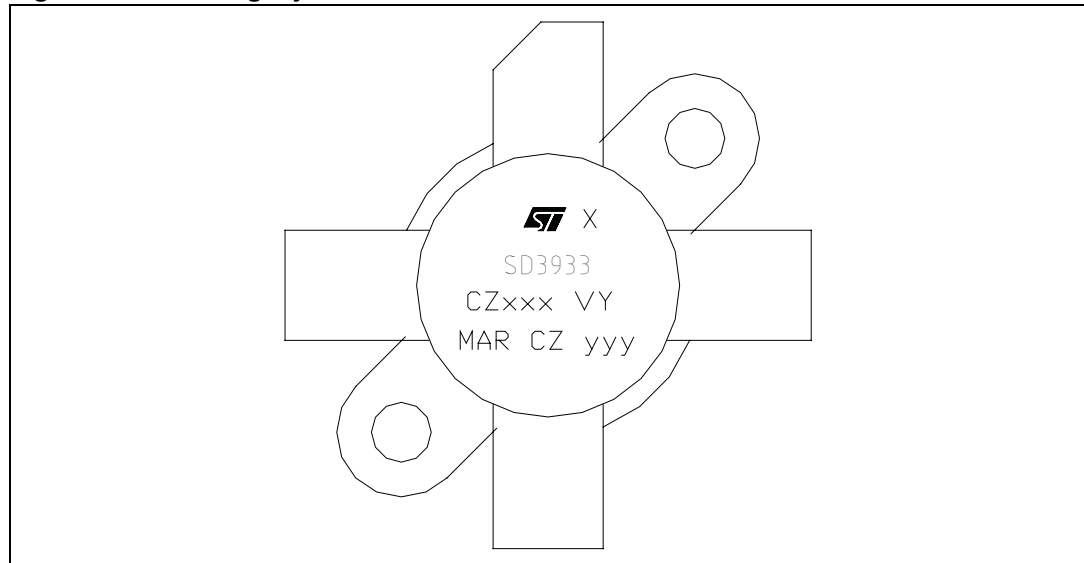
Figure 20. Marking layout
