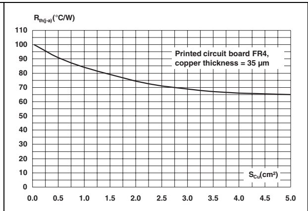
Figure 13. Thermal resistance junction to ambient versus lead copper surface under each lead
