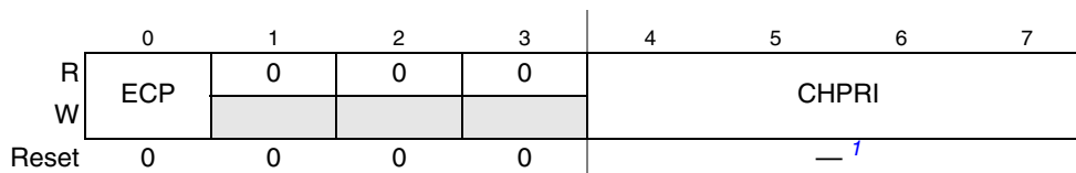
Figure 192. eDMA Channel n Priority Register (EDMA_CPR n )
