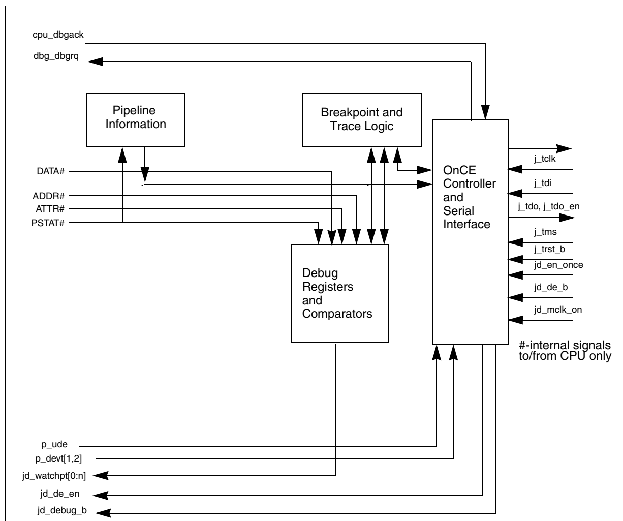
Figure 505. e200z0h Debug Resources
