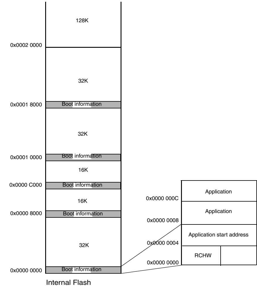
Figure 481. SPC560P40/34 Flash partitioning and RCHW search
