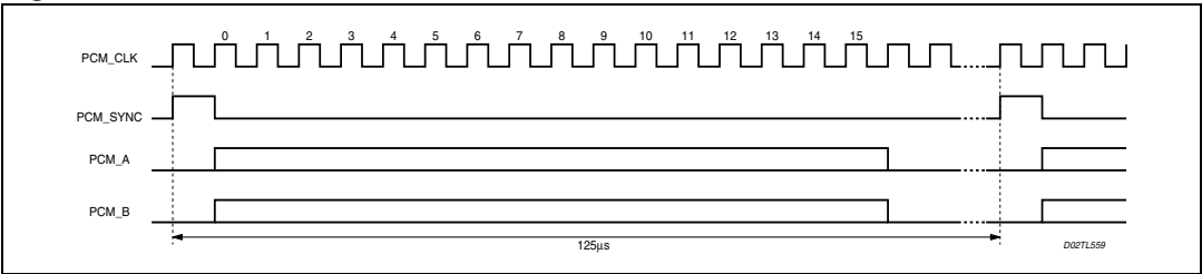
Figure 20. Linear mode
