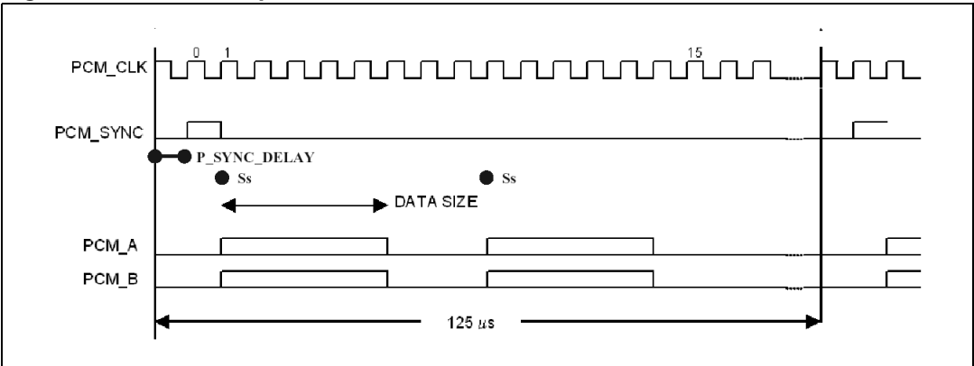
Figure 21. Multislot operation
