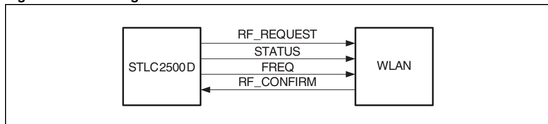
Figure 13. PTA diagram
